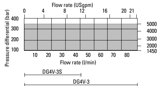
Typical maximum pressure differential (P-A-B-T) flow envelope, blocked center spool.
