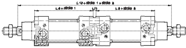
RA/8000/IT, RA/8000/MT – Four position cylinders
