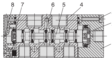
5/3 Ways Solenoid Valve
