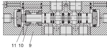
5/3 Ways Solenoid Valve
